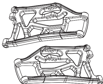
50 040 5263 Querlenker vorne/unten L/R Front lower suspension arm l/r
