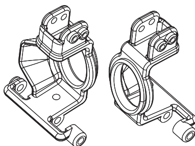
50 040 5263 Querlenker vorne/unten L/R Front lower suspension arm l/r
