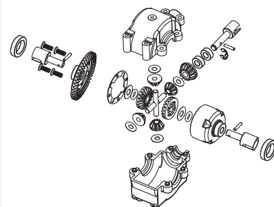
50 040 5283 Differenzial komplett Differential unit
